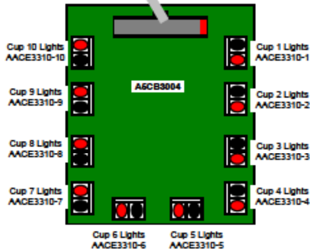
Playfield Layout for Cup Lights
