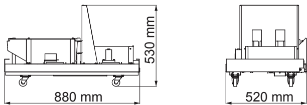
Hopper assembly
