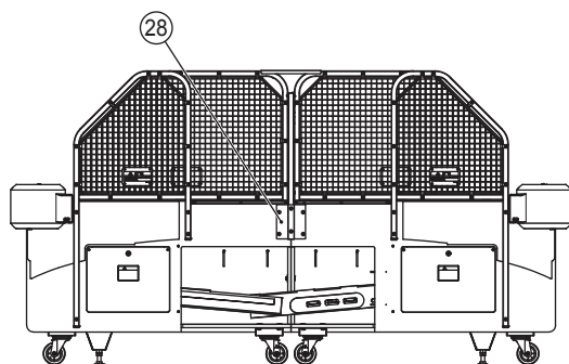
(View with the side tower assembly removed)
