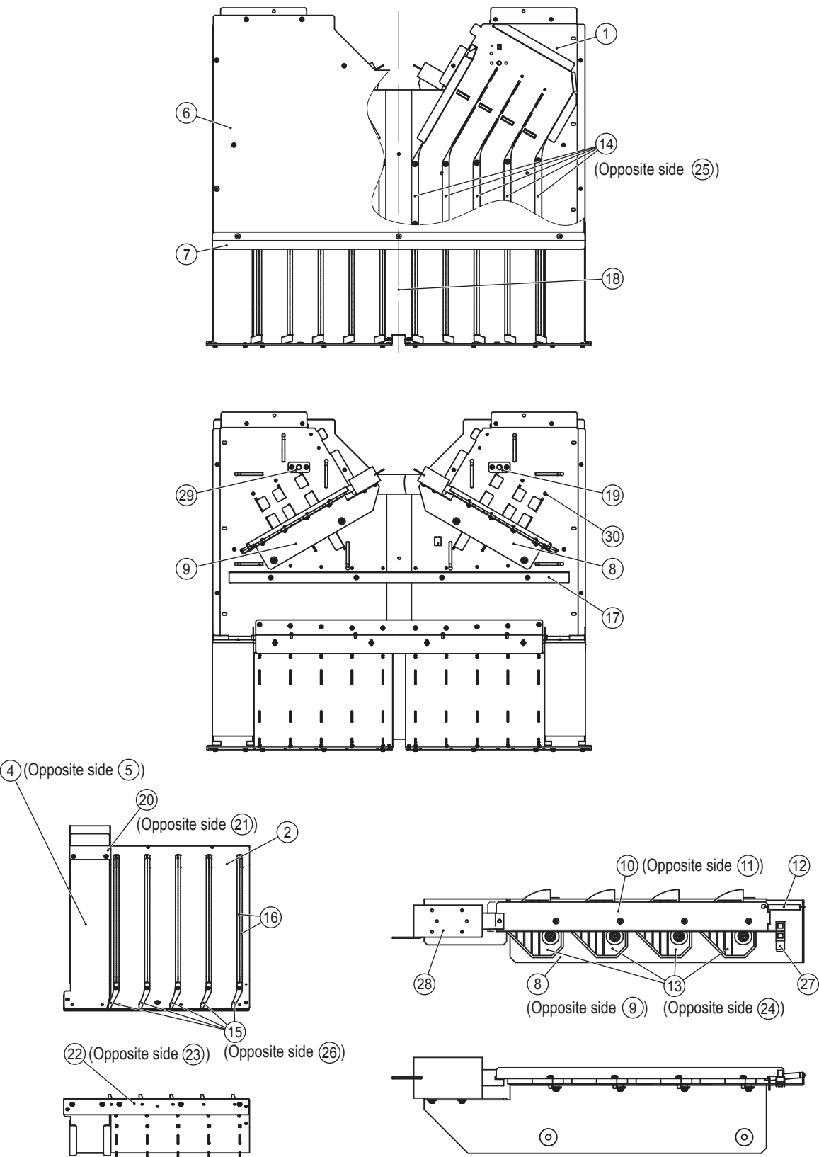
Detailed view of 2 and 3 (The figure shows 2.)
