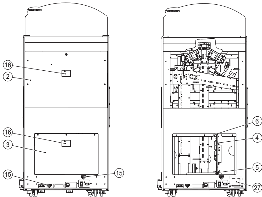
View with (2) and (3) removed
