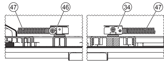
Cross-sectional diagram C-C (Condition with (27) removed)
