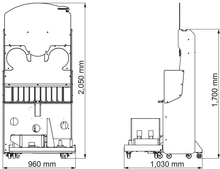
Hopper assembly
