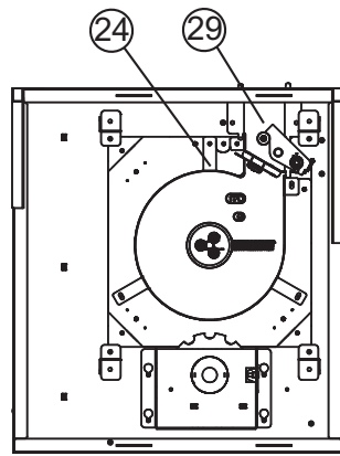
Condition with 4, 12, Y removed
